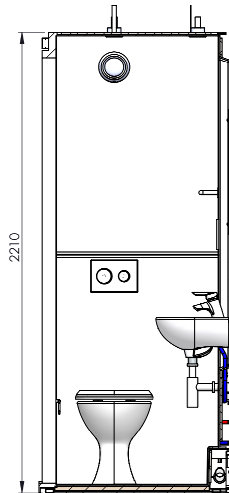
SECTION G-G
