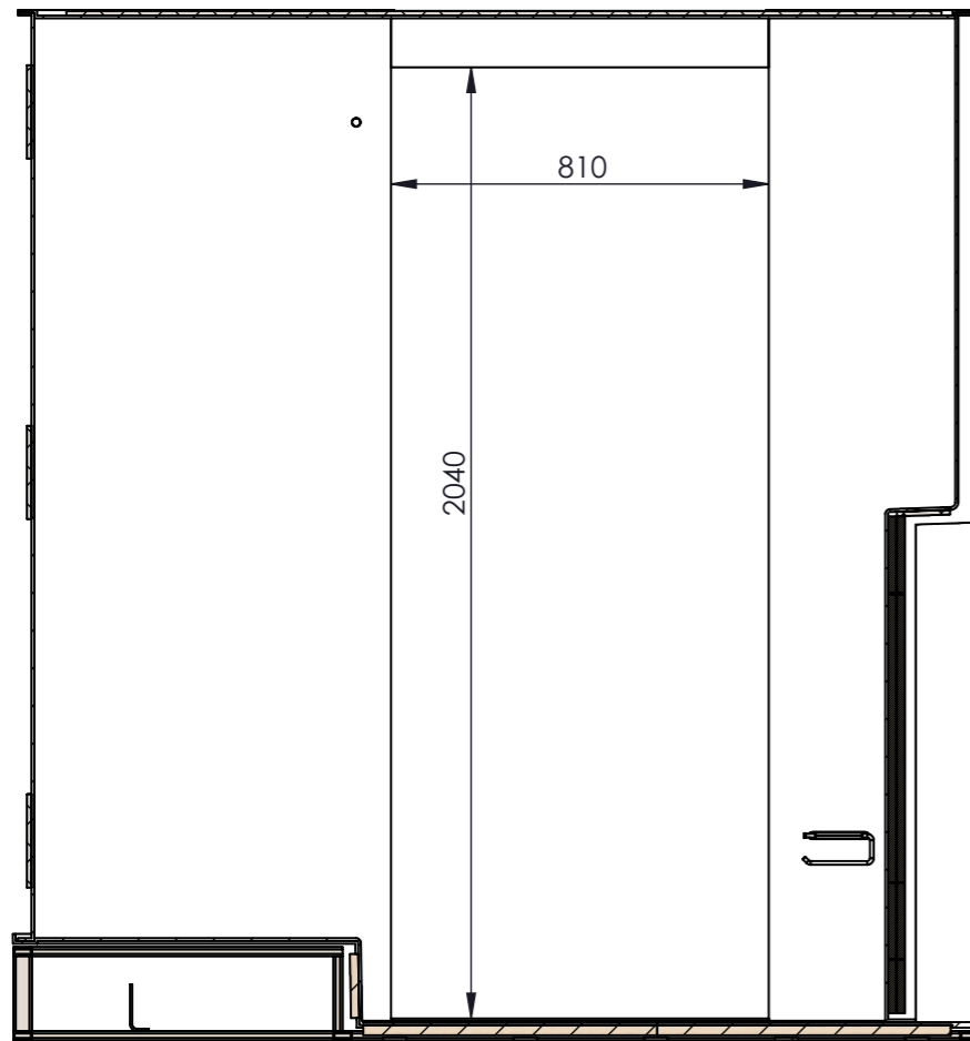
SECTION F-F
